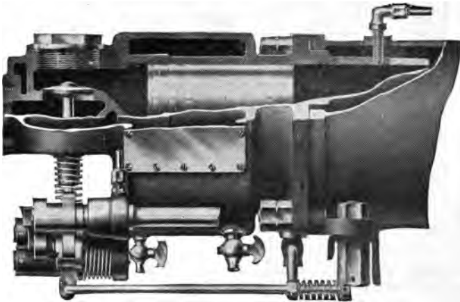
FIG. 239.—Part Sectional View of the Olds Motor, showing valve-operating mechanism. The cam-shaft, extending horizontally to the head of the motor, actuates a rocking cam, which in turn pushes both the inlet and exhaust valve stems, projecting below the motor head. The cam-shaft is rotated by a helical gear from the main shaft of the engine.
